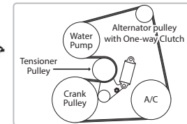
ENGINE ZD30D15 WITH 7PK AUTO-TENSIONED DRIVE BELT SYSTEM.
