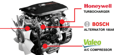
ENGINE ZD30D15 WITH 7PK AUTO-TENSIONED DRIVE BELT SYSTEM.
